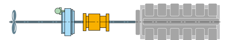
Single screw and PSC with secondary PTO* or PTH**
